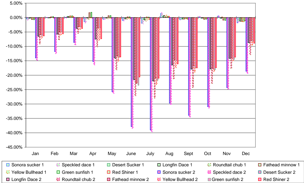
Figure 60. Average monthly change in habitat area (lowest 10 consecutive days) for the Braided site, with no LWD and with a hypothetical withdrawal of 2 ft 3 /s.
