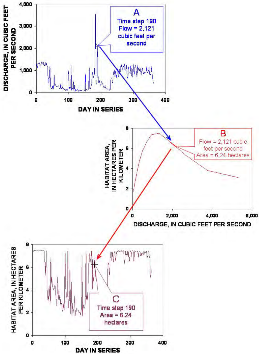
Figure 19. Elements used in the construction of a habitat time series, A flow time series, B Habitat-discharge function, and C the resulting habitat time series. From Bovee and others, 2008.
