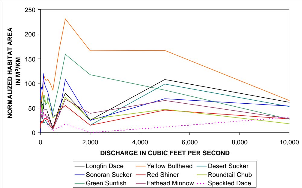
Figure 46. Habitat-discharge chart for the Gage site, with LWD in the habitat calculation, for the full range of simulated flows.
