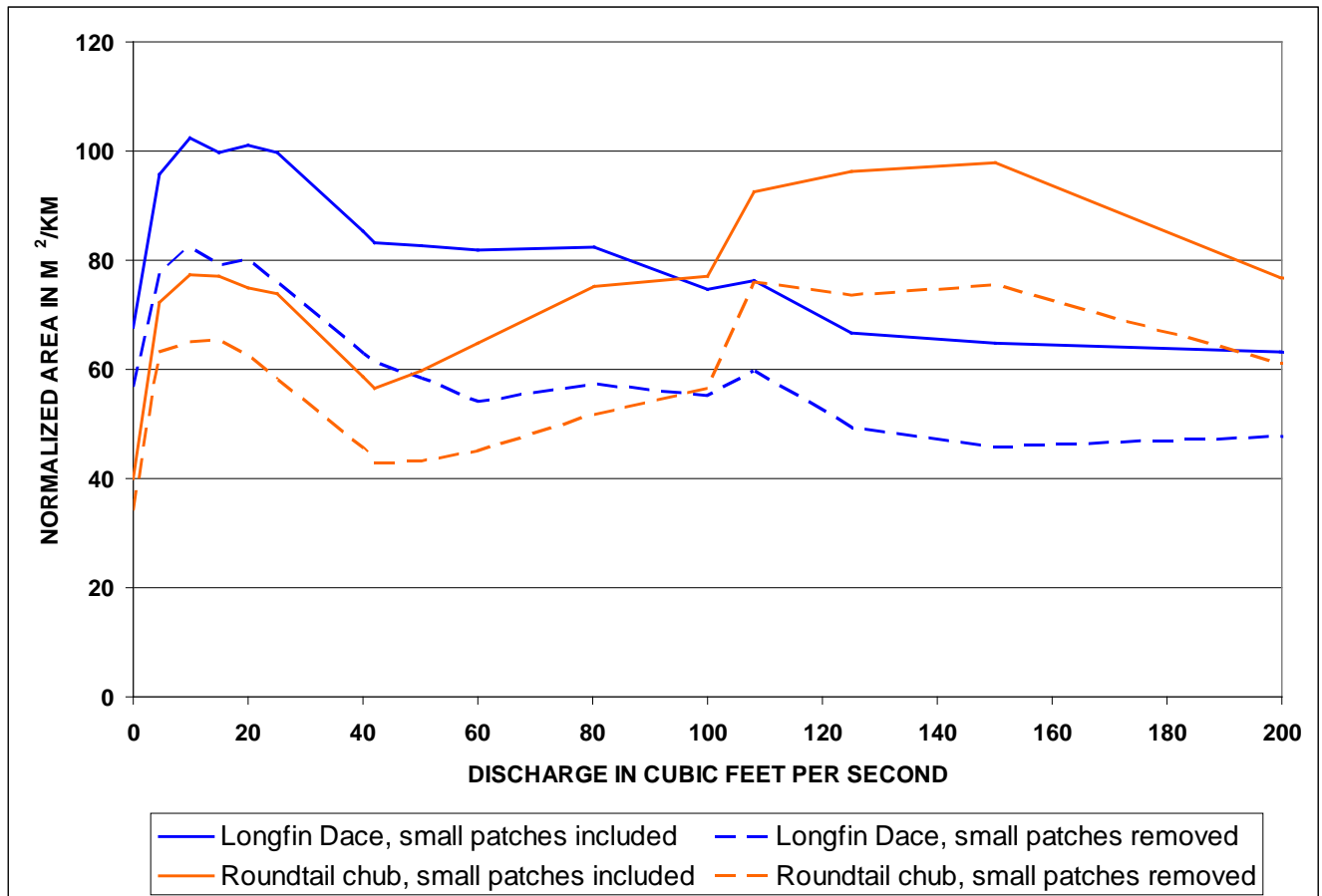
Figure 18. Effects of removing patches less than 0.1 m 2 in area on the habitat-discharge functions for two species at the Gage site, with LWD included in the habitat computations.
