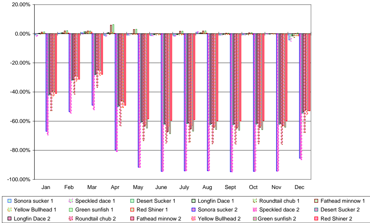
Figure 61. Average monthly change in habitat area (lowest 10 consecutive days) for the Braided site, with no LWD and with a hypothetical withdrawal of 10 ft 3 /s.
