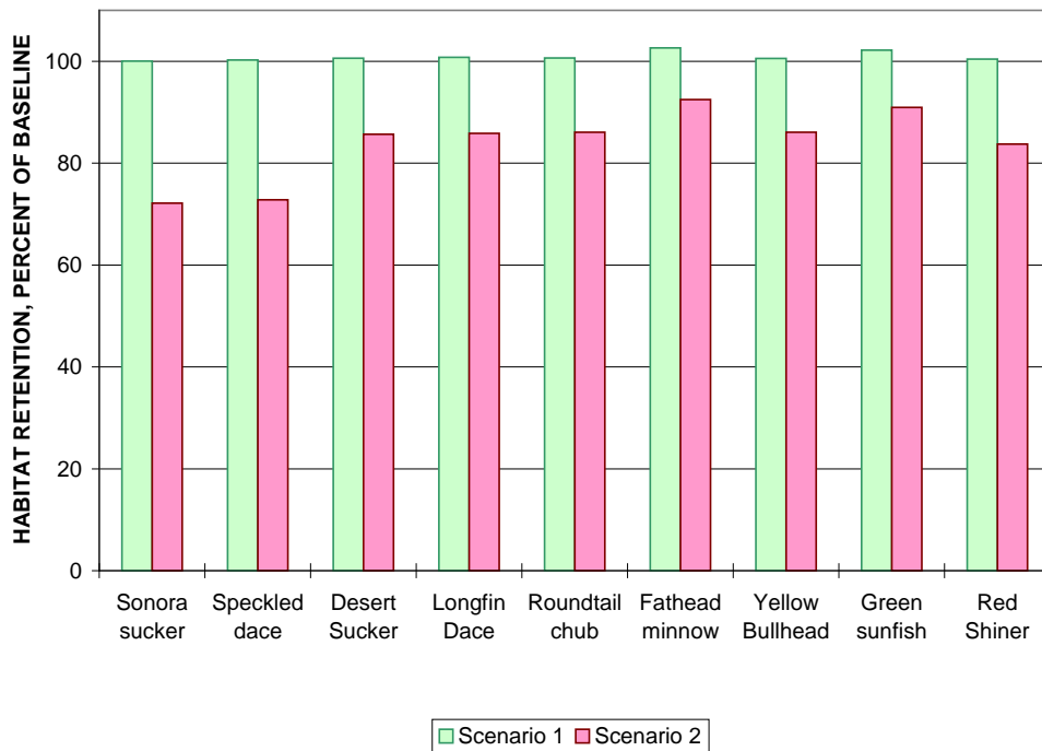
Figure 68. Habitat retention for the Gage site, without LWD and with a hypothetical withdrawal of 2 ft 3 /s.
