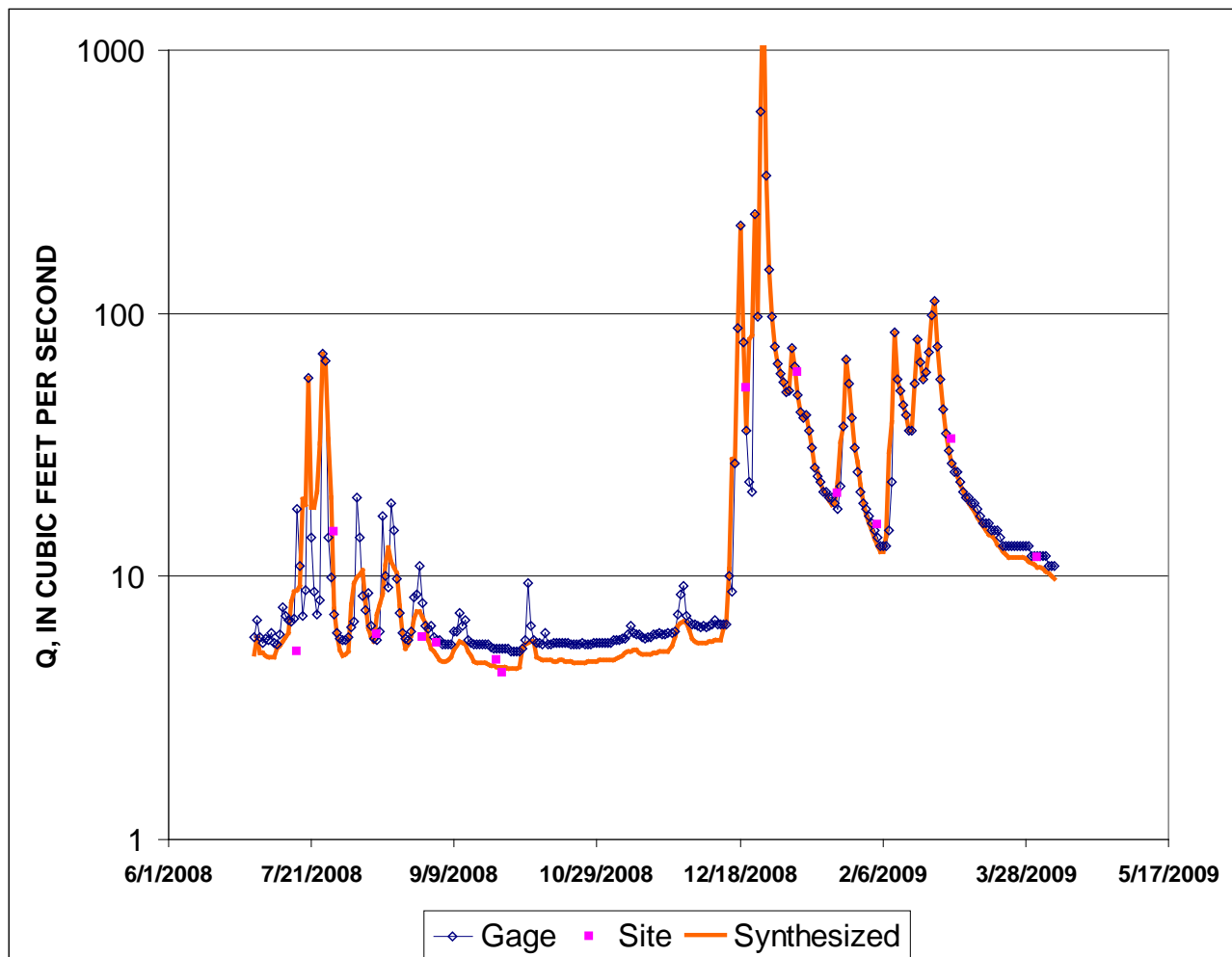
Figure 43. Synthesized daily discharge at the Braided site compared to onsite flow observations and Cherry Creek gage flows. The onsite observations indicate that flow at the Braided site is approximately the same as the gage above about 10 ft 3 /s and clearly lower than the gage at base flow.
