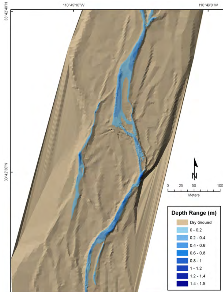
Figure 5. Depth TIN for the lower (Braided) site at Cherry Creek for a discharge of 10 ft 3 /sec.
