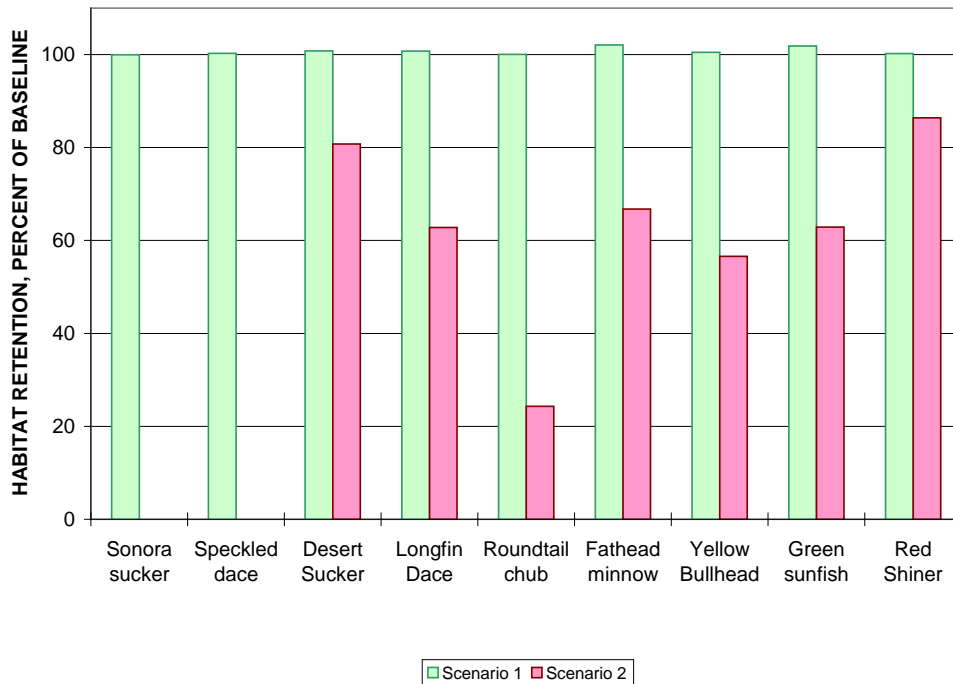
Figure 75. Habitat retention for the Braided site, with LWD and a hypothetical withdrawal of 10 ft 3 /s.
