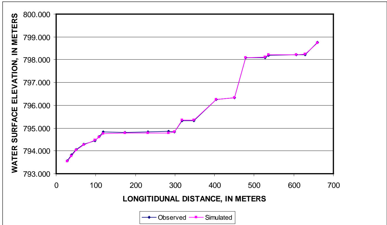
Figure 38. Observed and simulated water surface profiles for the Braided site at 0.137 \text{ m}^3/\text{s} ( 4.84 \text{ ft}^3/\text{s} ).
