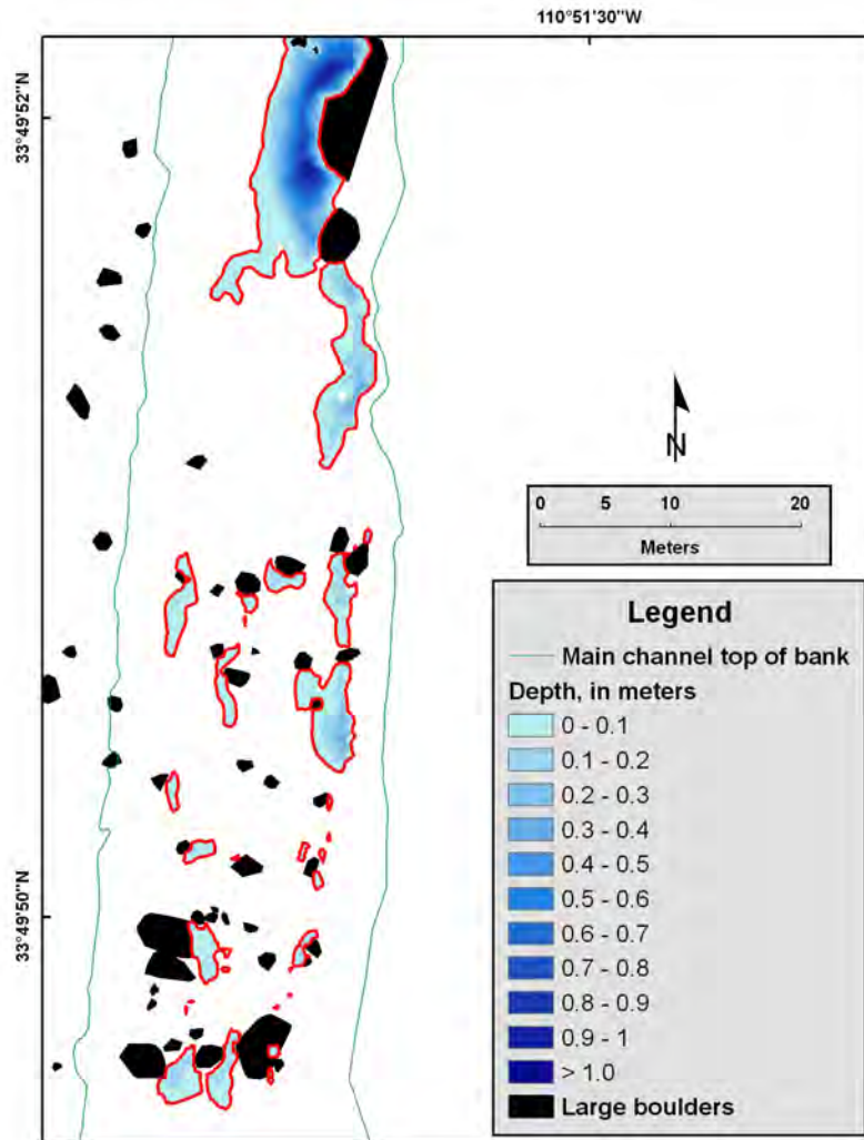
Figure 16. Map of a portion of the upper (Gage) site showing the depth distribution in isolated pools at zero discharge.
