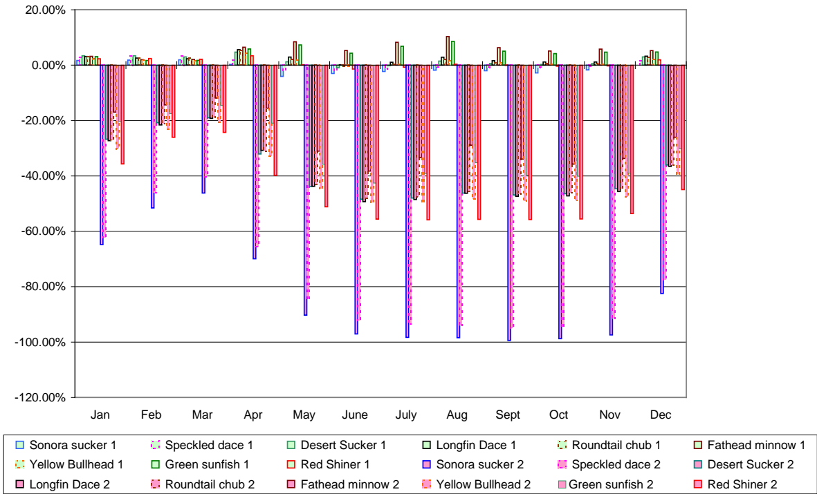
Figure 57. Average monthly change in habitat area (lowest 10 consecutive days) for the Gage site, with no LWD and with a hypothetical withdrawal of 10 ft 3 /s.
