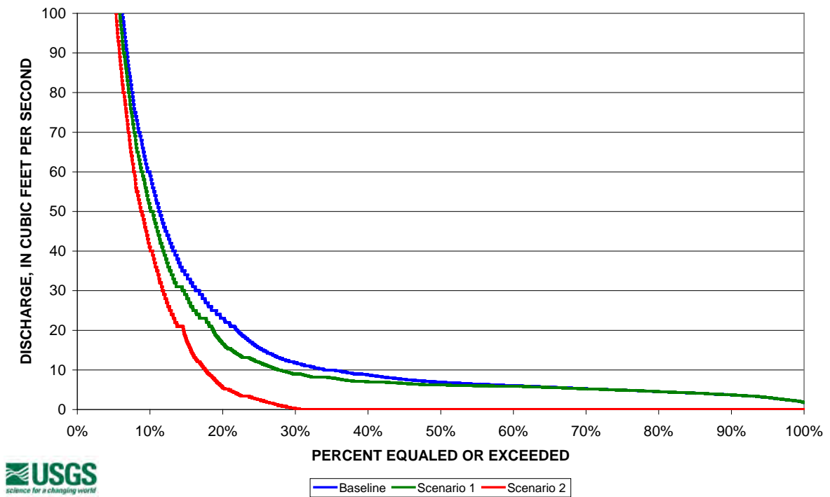
Figure 55. Flow duration curve for the Braided site under baseline conditions and scenarios 1 and 2, assuming a hypothetical diversion of 10 ft 3 /s.
