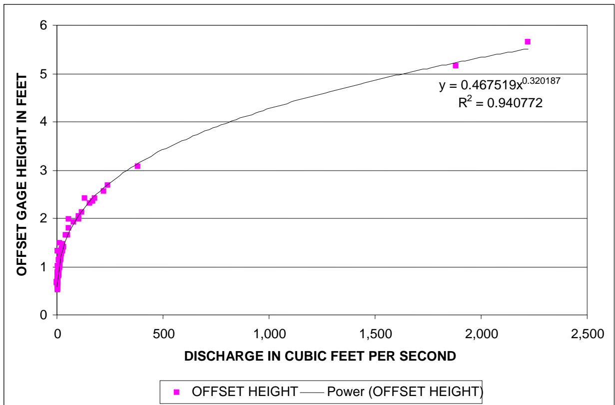
Figure 3. Observed gage height offset by -1.15 ft and power function fit.
