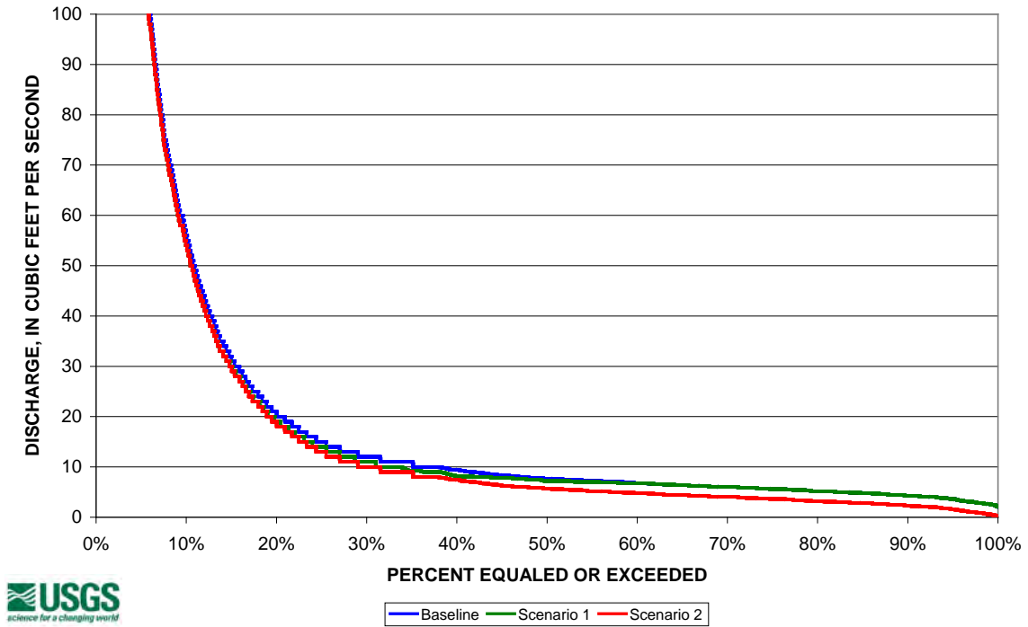
Figure 52. Flow duration curve for the Gage site under baseline conditions and scenarios 1 and 2, assuming a hypothetical diversion of 2 ft 3 /s.
