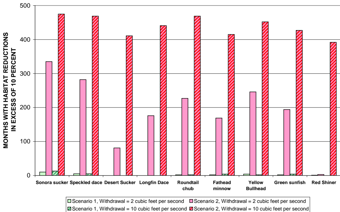
Figure 67. Count of months having a habitat reduction of 10 percent or more at the Braided site for the period of record, with LWD.
