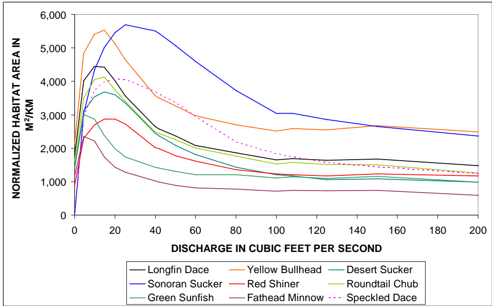
Figure 45. Habitat-discharge chart for the Gage site, without LWD in the habitat calculation, for flows between 0 and 200 ft³/s.
