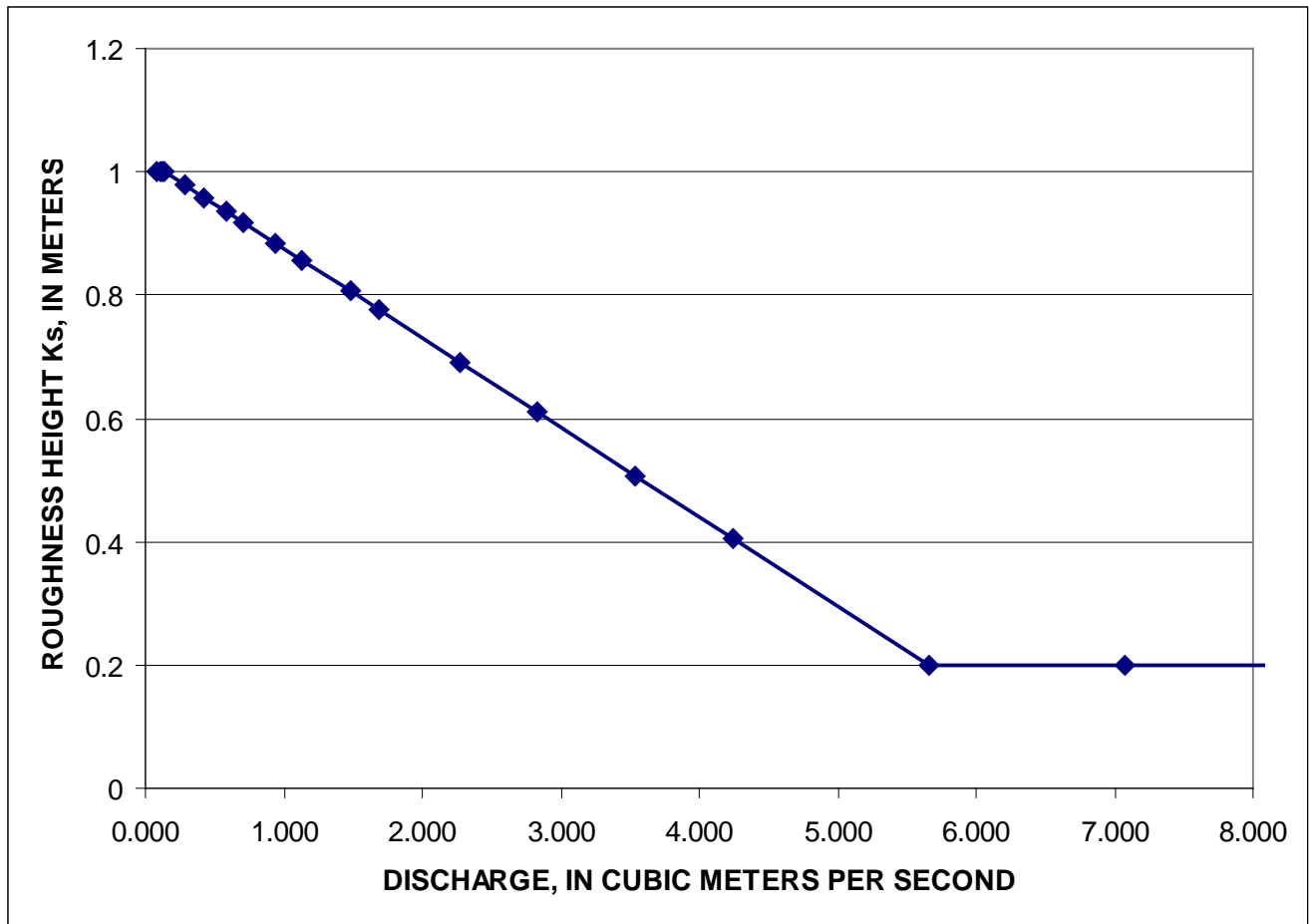
Figure 39. Braided site roughness height-discharge relation.
