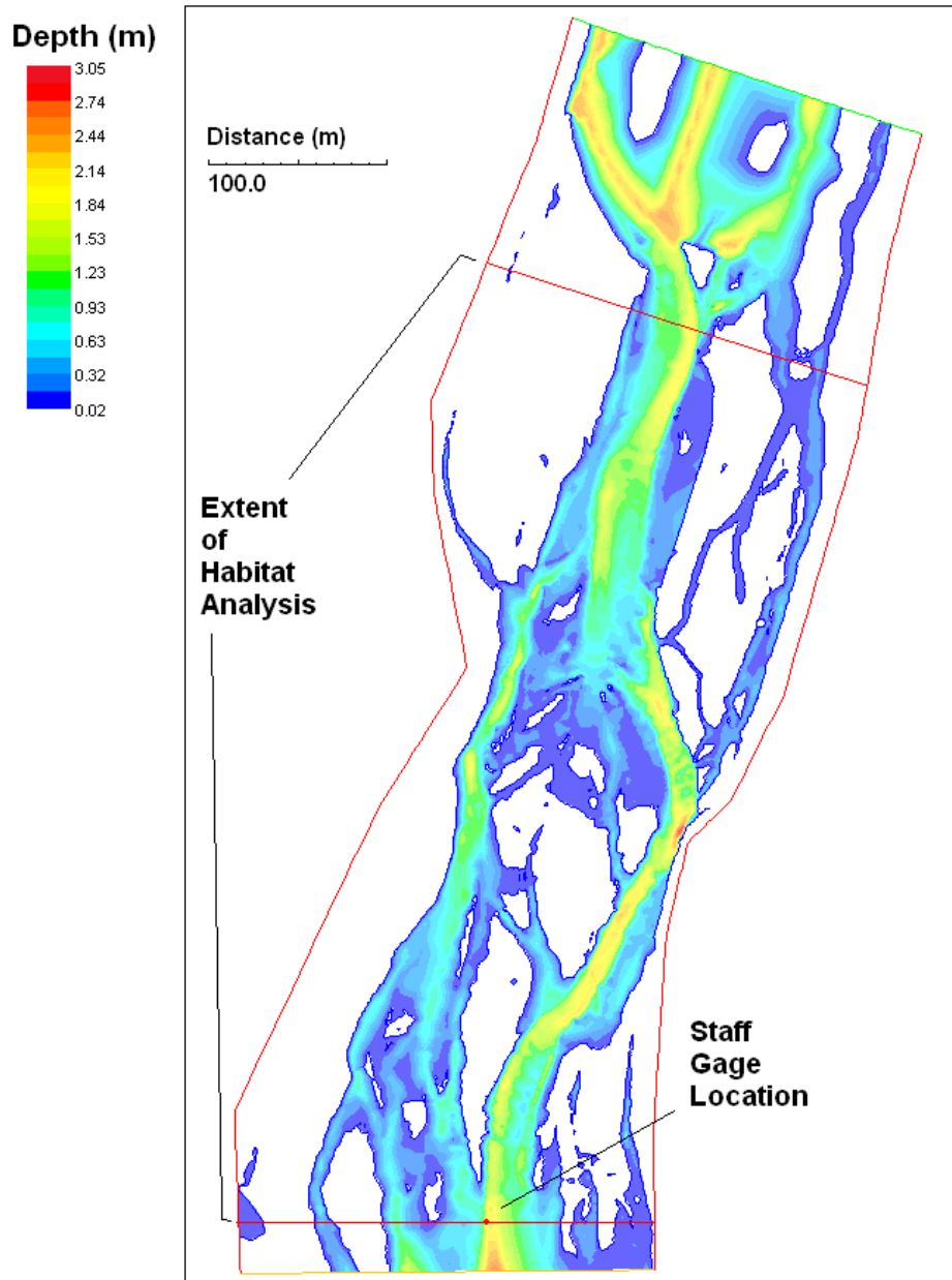
Figure 42. Depth distribution for Braided site for a simulated discharge of 3,800 ft 3 /s (107.8 m 3 /s)
