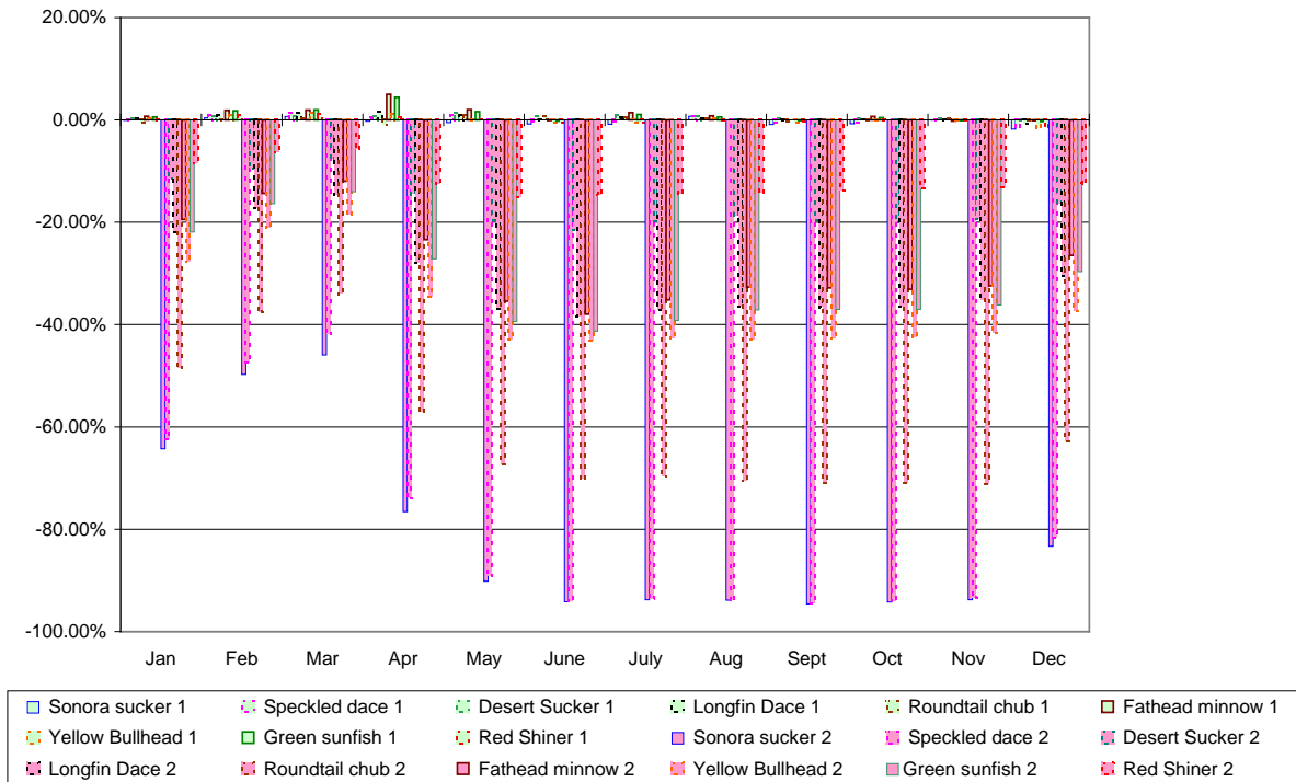
Figure 63. Average monthly change in habitat area (lowest 10 consecutive days) for the Braided site, with LWD and a hypothetical withdrawal of 10 ft 3 /s.
