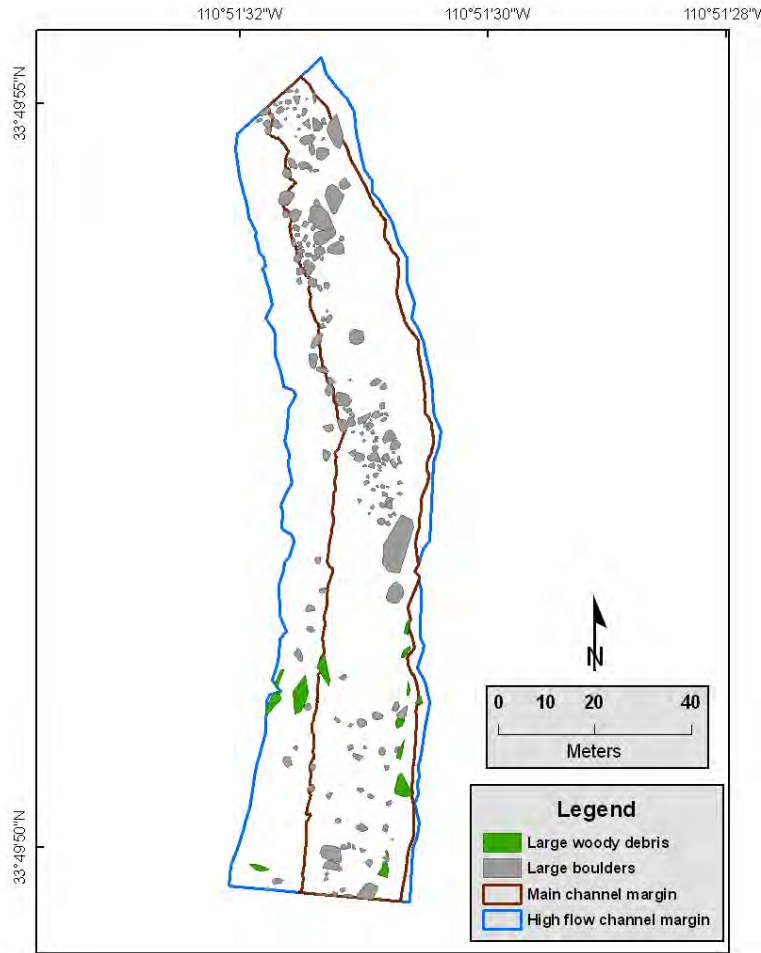
Figure 14. LWD polygons for the upper (Gage) site resulting from application of the convex hull algorithm to survey points outlining individual root wads or debris deposits.
