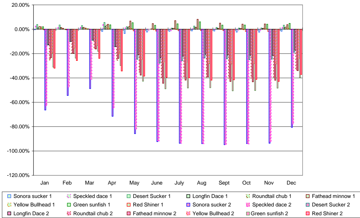
Figure 59. Average monthly change in habitat area (lowest 10 consecutive days) for the Gage site, with LWD and a hypothetical withdrawal of 10 ft 3 /s.
