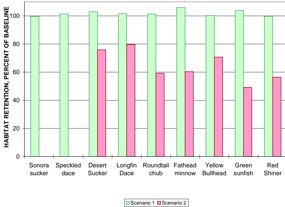
Figure 71. Habitat retention for the Gage site, with LWD and with a hypothetical withdrawal of 10 ft 3 /s.
