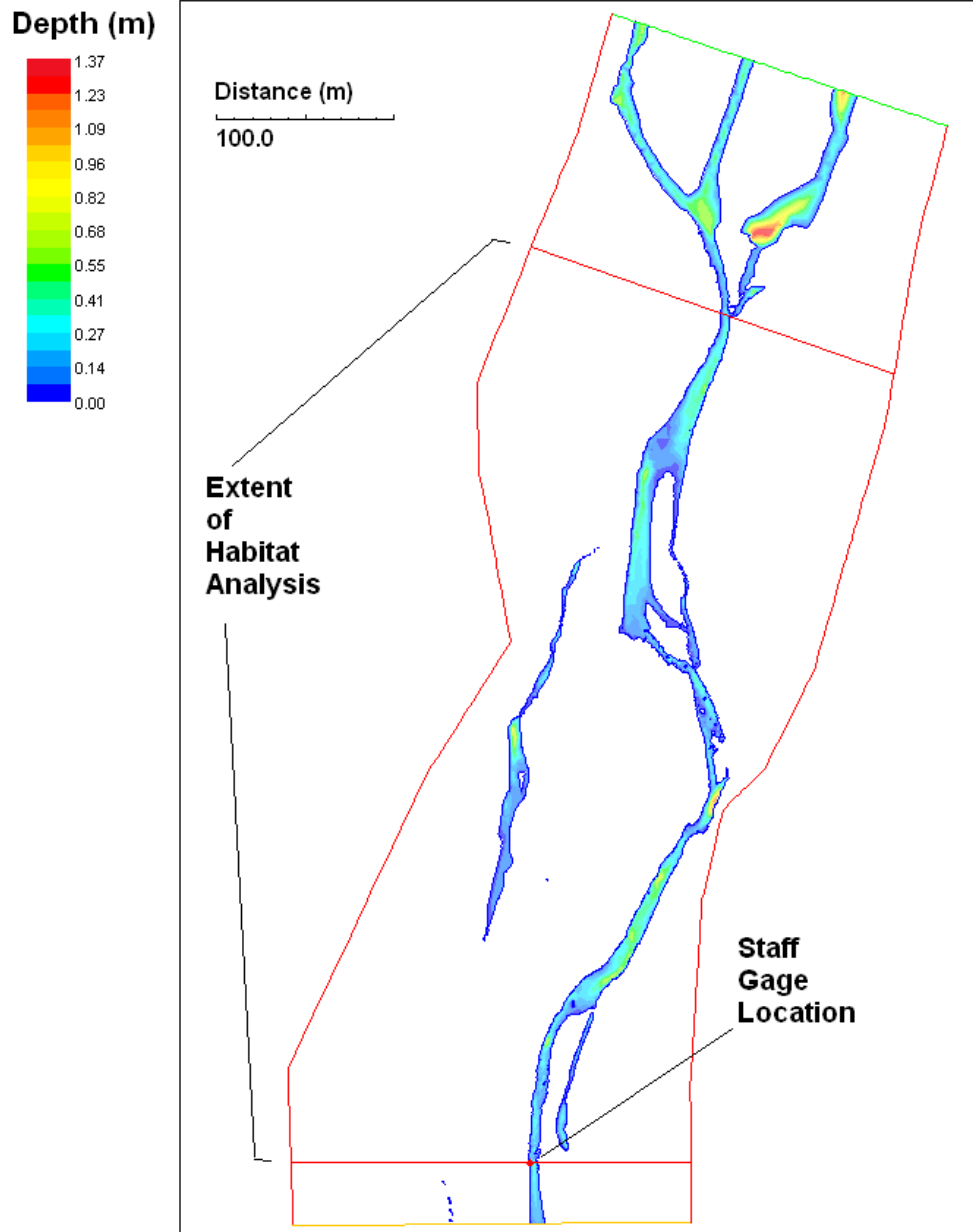
Figure 41. Depth distribution at Braided site for the 0.137 m 3 /s (4.84 ft 3 /s) discharge.
