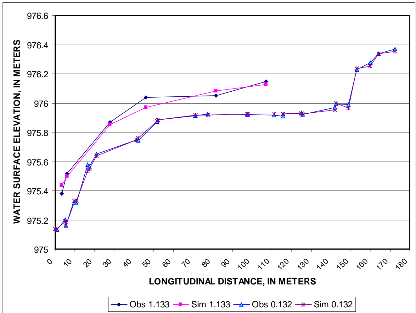
Figure 37. Observed (Obs) and simulated (Sim) water surface profiles for the Gage site at discharges of 0.132 and 1.133 m 3 /s (4.65 and 40 ft 3 /s).
