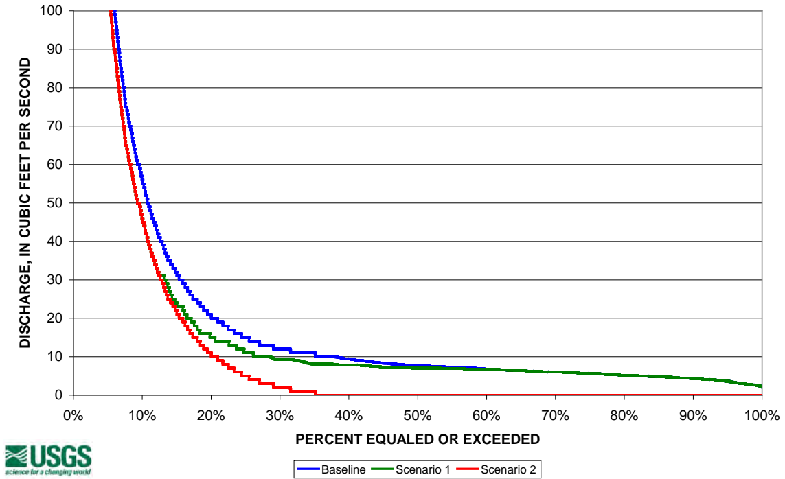
Figure 54. Flow duration curve for the Gage site under baseline conditions and scenarios 1 and 2, assuming a hypothetical diversion of 10 ft 3 /s.
