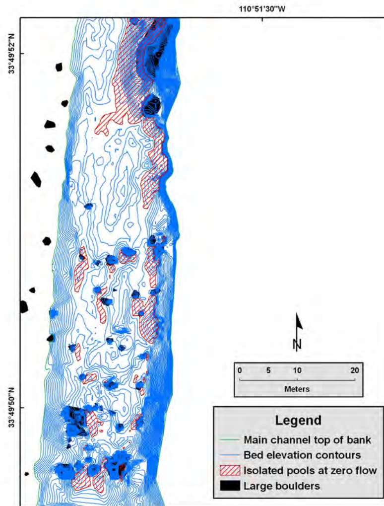
Figure 15. Map of a portion of the upper (Gage) site showing bed elevation contours and closed contours representing the stage of zero flow for isolated pools.
