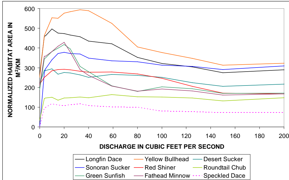
Figure 51. Habitat-discharge chart for the Braided site, with LWD in the habitat calculation, for flows between 0 and 200 ft 3 /s.
