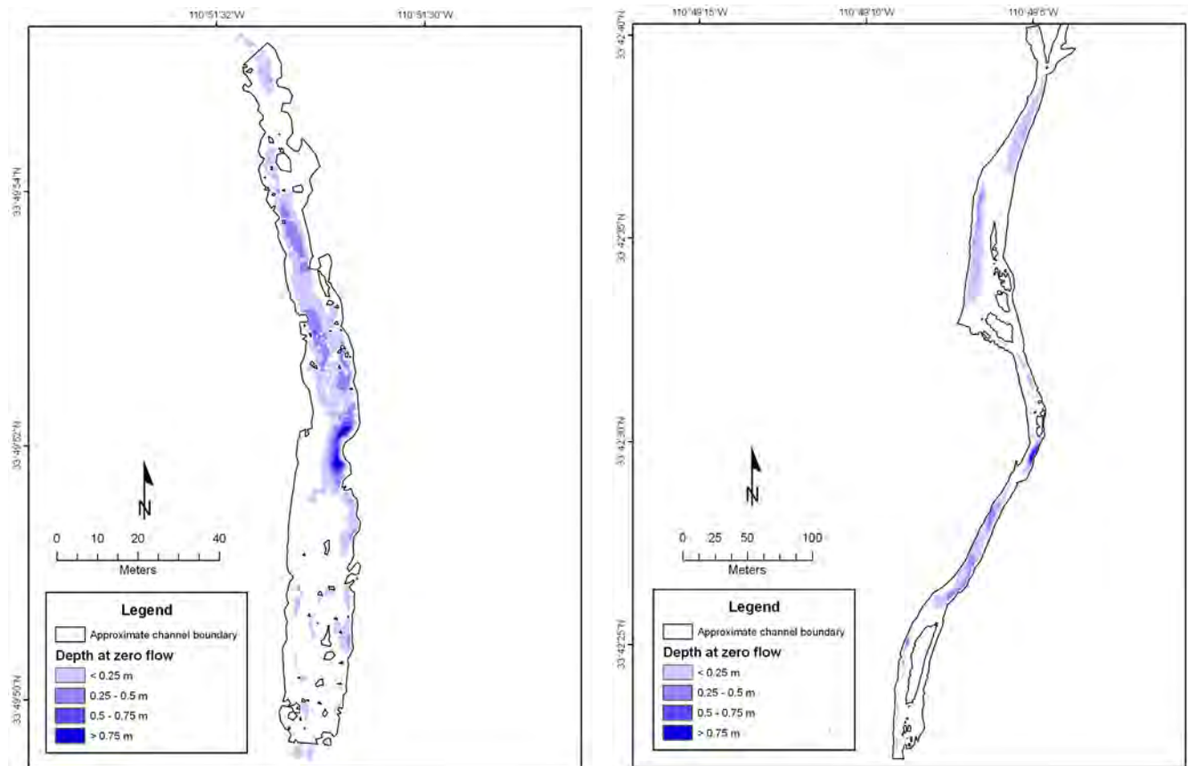
Figure 77. Depths of pools at zero discharge in the Gage site (left) and Braided site (right).
