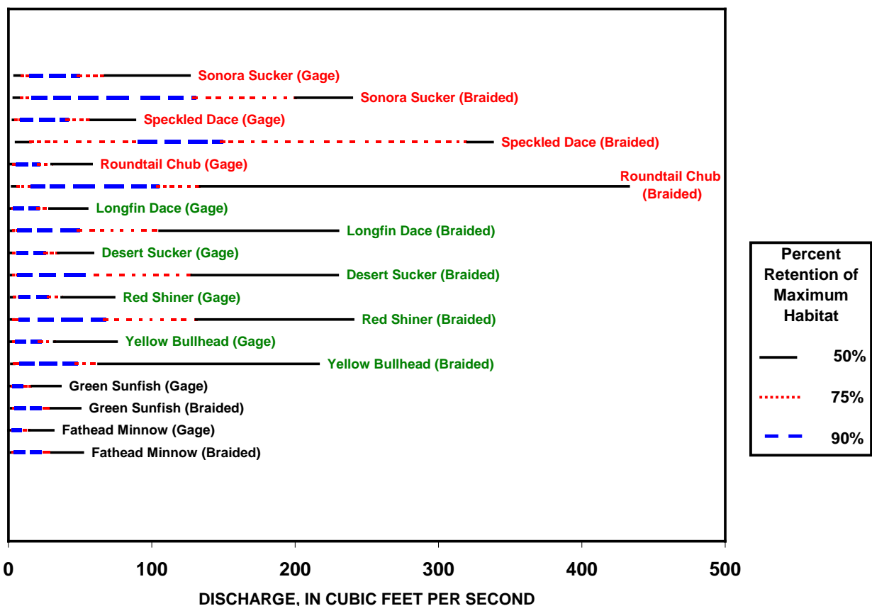
Figure 76. Ranges of discharges providing 50 percent, 75 percent, and 90 percent of the habitat maxima for all target species at both Cherry Creek study sites. Data labels for Group 1 are in red typeface, Group 2 in green typeface, and Group 3 in black typeface.
