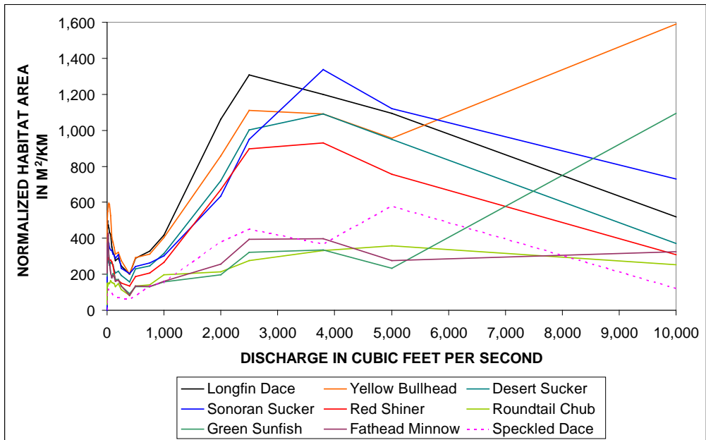
Figure 50. Habitat-discharge chart for the Braided site, with LWD in the habitat calculation, for the full range of simulated flows.
