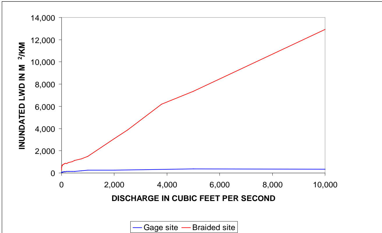
Figure 78. Inundation of LWD as a function of discharge at the two study sites.
