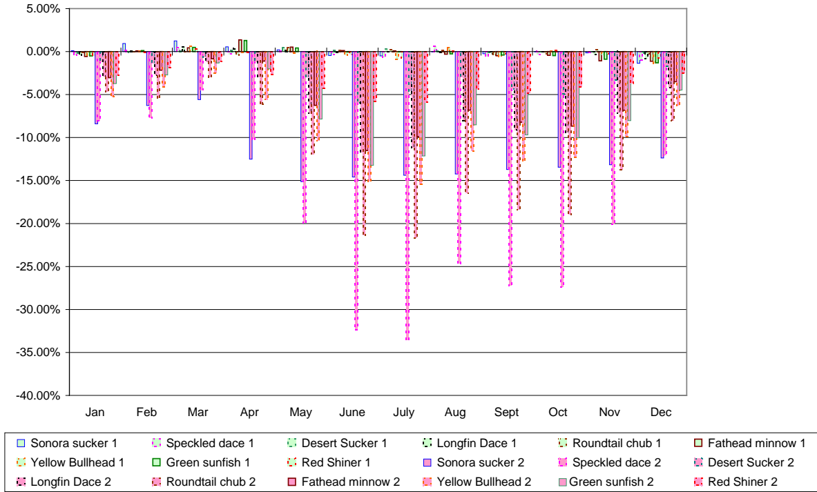
Figure 62. Average monthly change in habitat area (lowest 10 consecutive days) for the Braided site, with LWD and a hypothetical withdrawal of 2 ft 3 /s.
