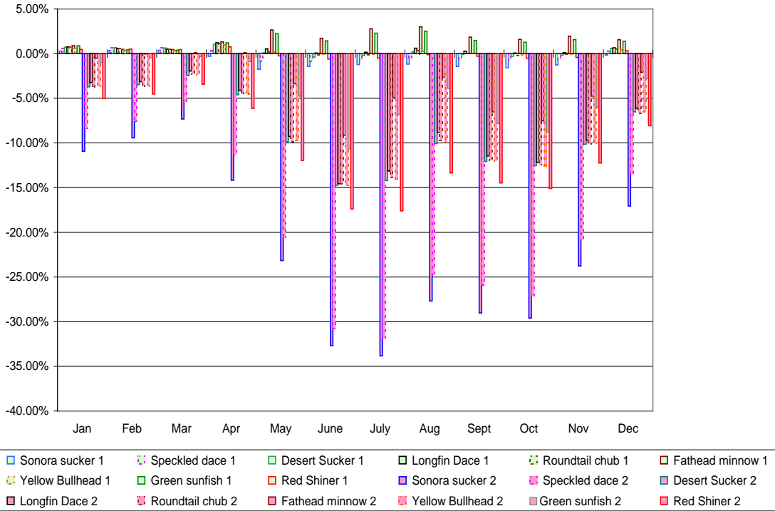
Figure 56. Average monthly change in habitat area (lowest 10 consecutive days) for the Gage site, with no LWD and with a hypothetical withdrawal of 2 ft 3 /s.
