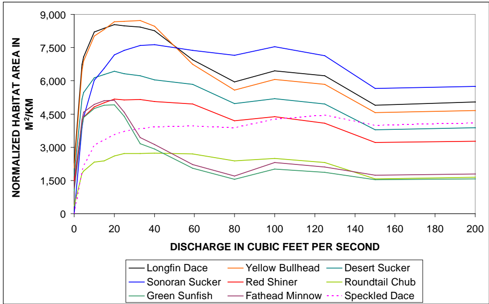
Figure 49. Habitat-discharge chart for the Braided site, without LWD in the habitat calculation, for flows between 0 and 200 ft 3 /s.
