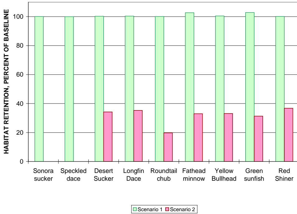
Figure 73. Habitat retention for the Braided site, without LWD and with a hypothetical withdrawal of 10 ft 3 /s.
