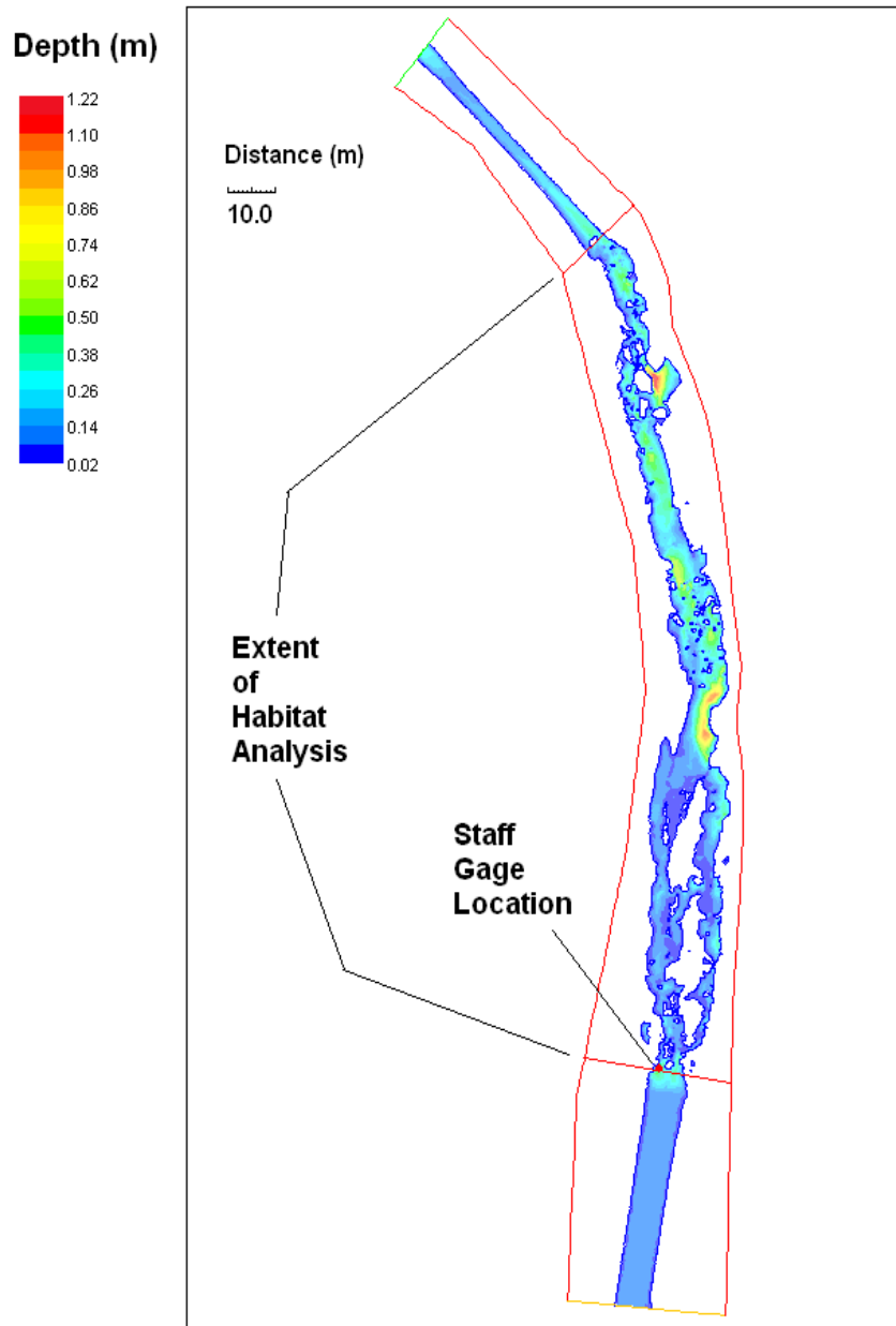
Figure 40. Depth distribution at Gage site for the 0.132 m 3 /s (4.67 ft 3 /s) discharge.
