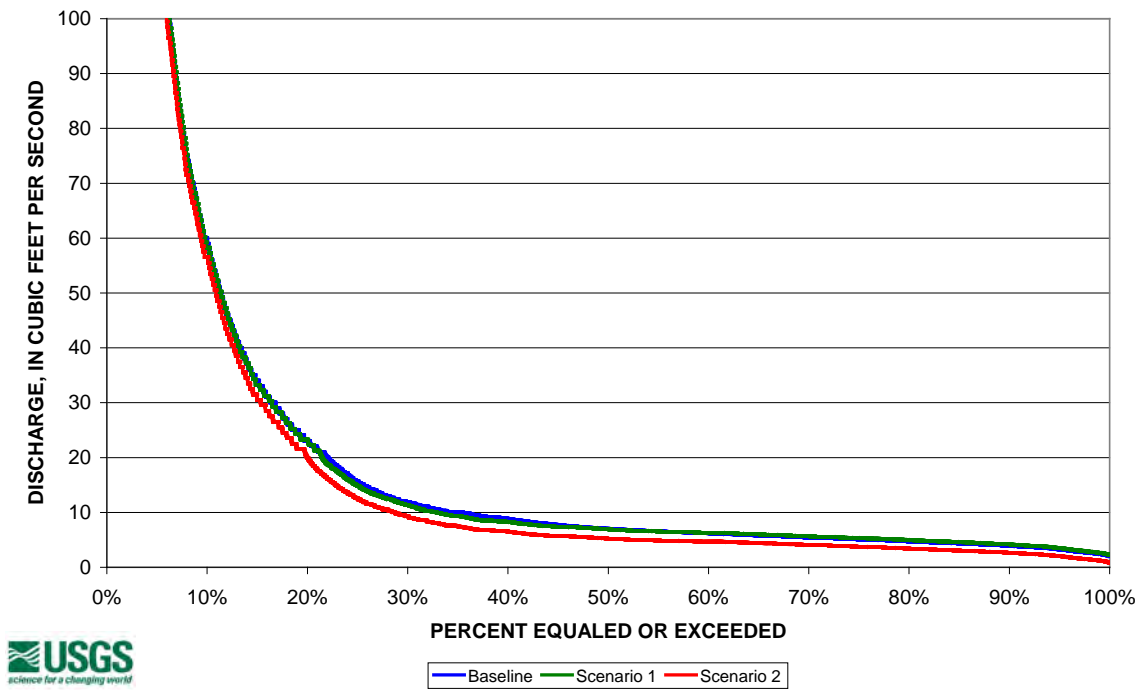
Figure 53. Flow duration curve for the Braided site under baseline conditions and scenarios 1 and 2, assuming a hypothetical diversion of 2 ft 3 /s.
