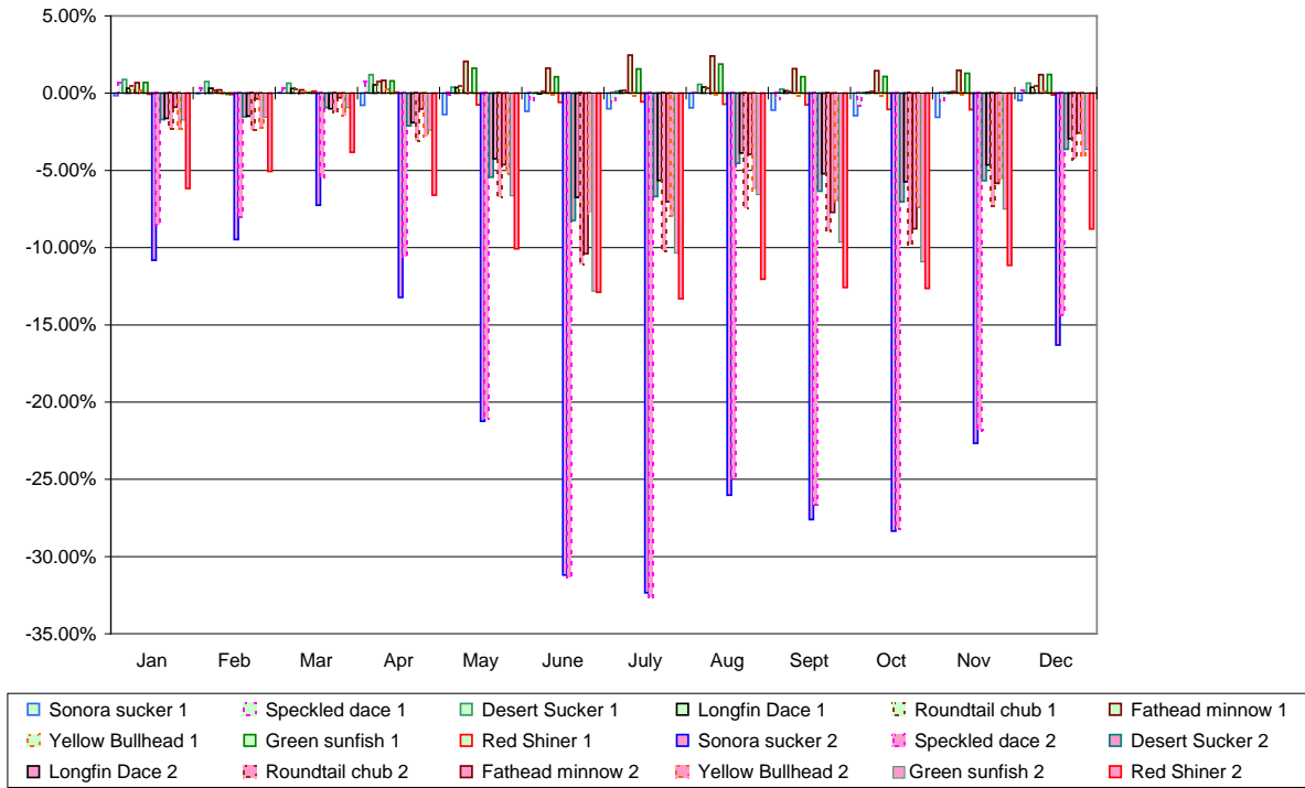
Figure 58. Average monthly change in habitat area (lowest 10 consecutive days) for the Gage site, with LWD and a hypothetical withdrawal of 2 ft 3 /s.
